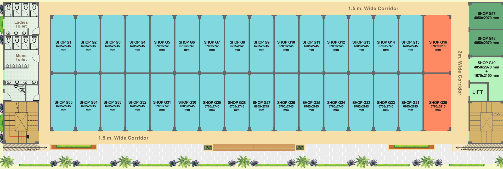
GROUND FLOOR PLAN COMMERCIAL - 1
