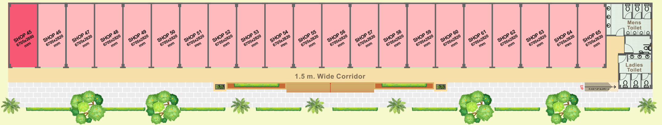
GROUND FLOOR PLAN COMMERCIAL - 3 Global City Centre 88A
